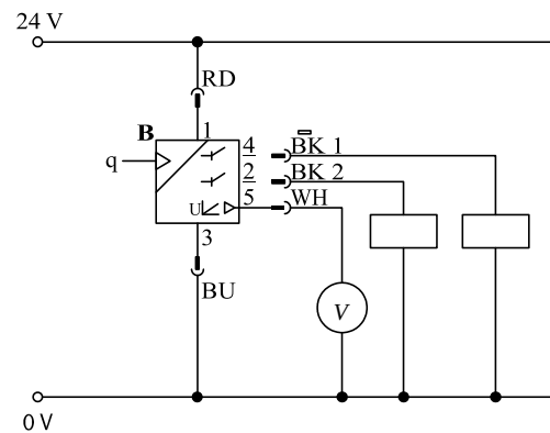
Rys. 2.5 Flow measuring range 0,5 – 50 l/min, Symbol, Electrical connection of the flow sensor
