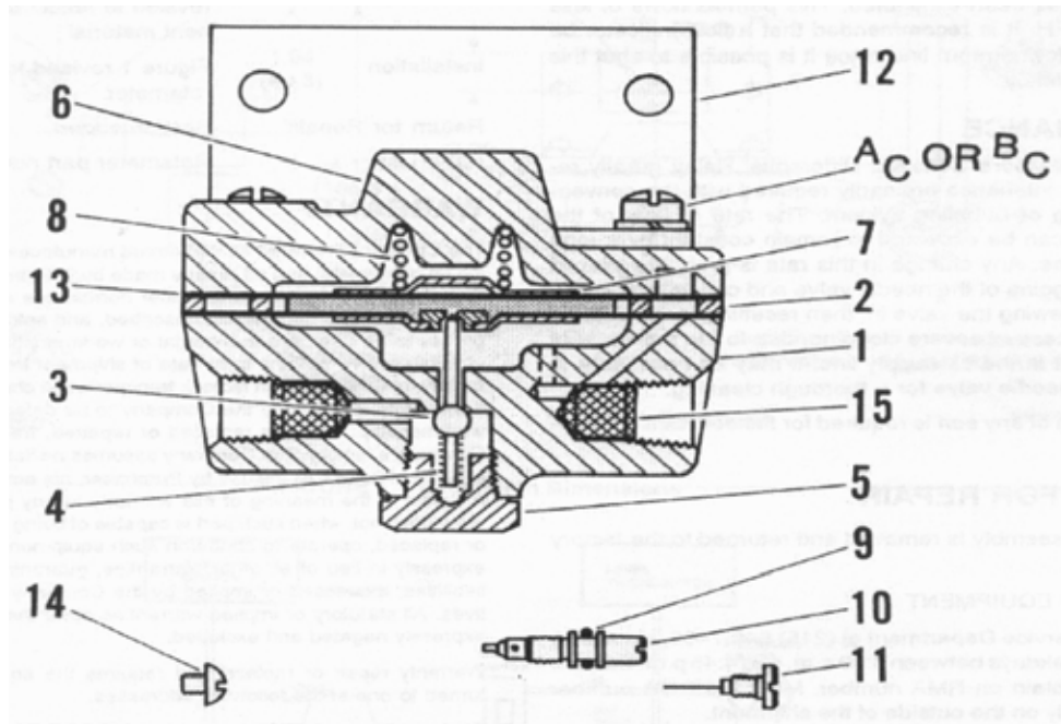
Rys. 10 Regulator małych przepływów: Siemens model series 62 Constant Differential Relay. Parts: 1-bottom forging, 2-exhaust diaphragm assy, 3-plunger assy, 4-valve spring, 5-retaining nut, 6-top forging, 7- diaphragm disc, 8-differential spring, 9-o ring. 10-restriction screw, 11-cleaning wire, 12 mounting bracket, 13-diaphragm, 14-retaining screw, 15 filter screens.
