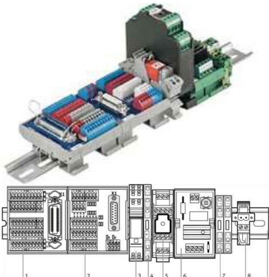
Rys. 2.3 Elementy sterowania - 1: I/O terminal XD1; 2: analogue terminal XD3; 3: relay, 2 switch-over contacts KF1; 4: relay, 1 switch-over contact KF2; 5: motor controller QA1; 6: starting current limiter QA0; 7: PE terminals XE0; 8: motor terminal XD20; 9: top hat rail
